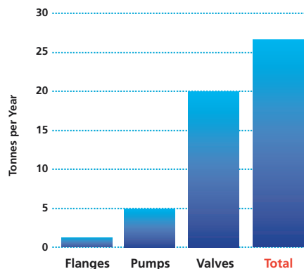
Properly assembled flanged joints have little overall impact on total emissions
